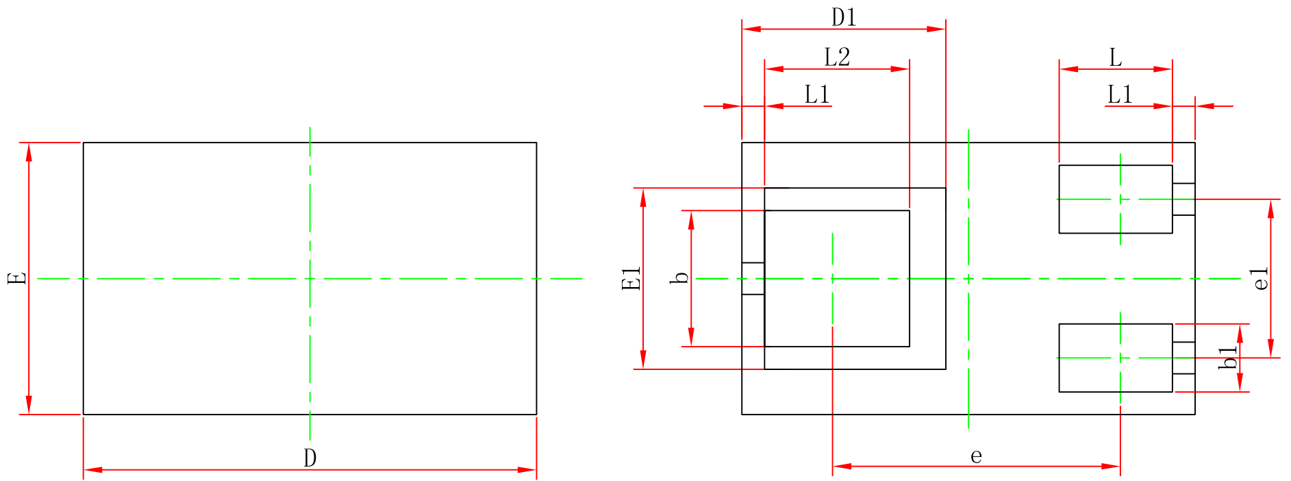
BOTTOM VIEW
