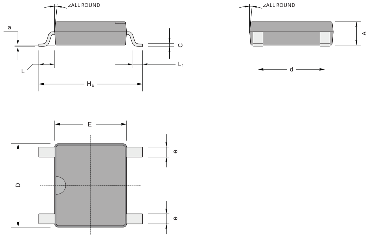
ABS/LBF mechanical data
